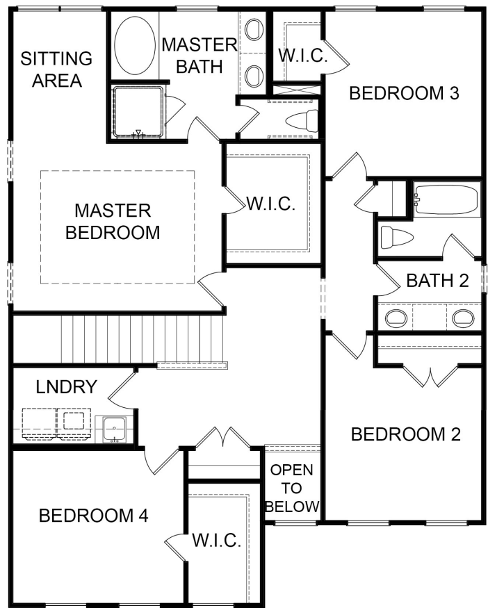
Second Floor
